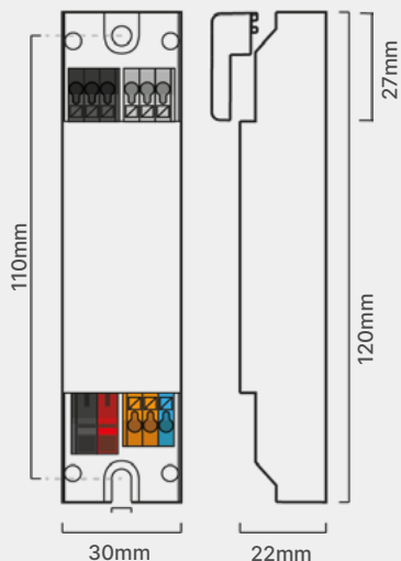
30mm casing with strain relief for suspended ceilings
