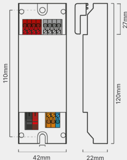
42mm casing with strain relief for suspended ceilings
